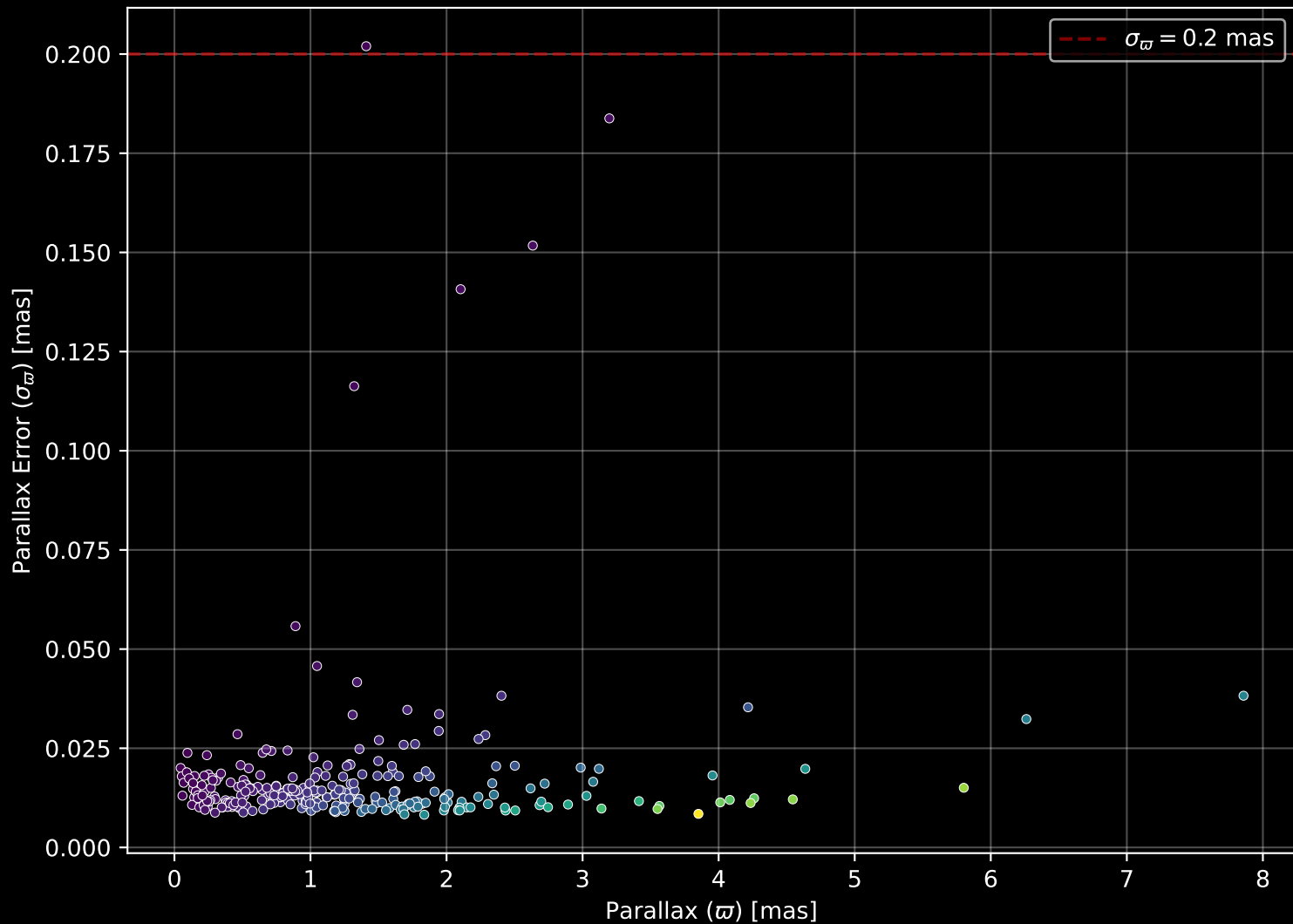
APOGEE DR17 Field: [255-27] Parallax Quality (n= 283)
