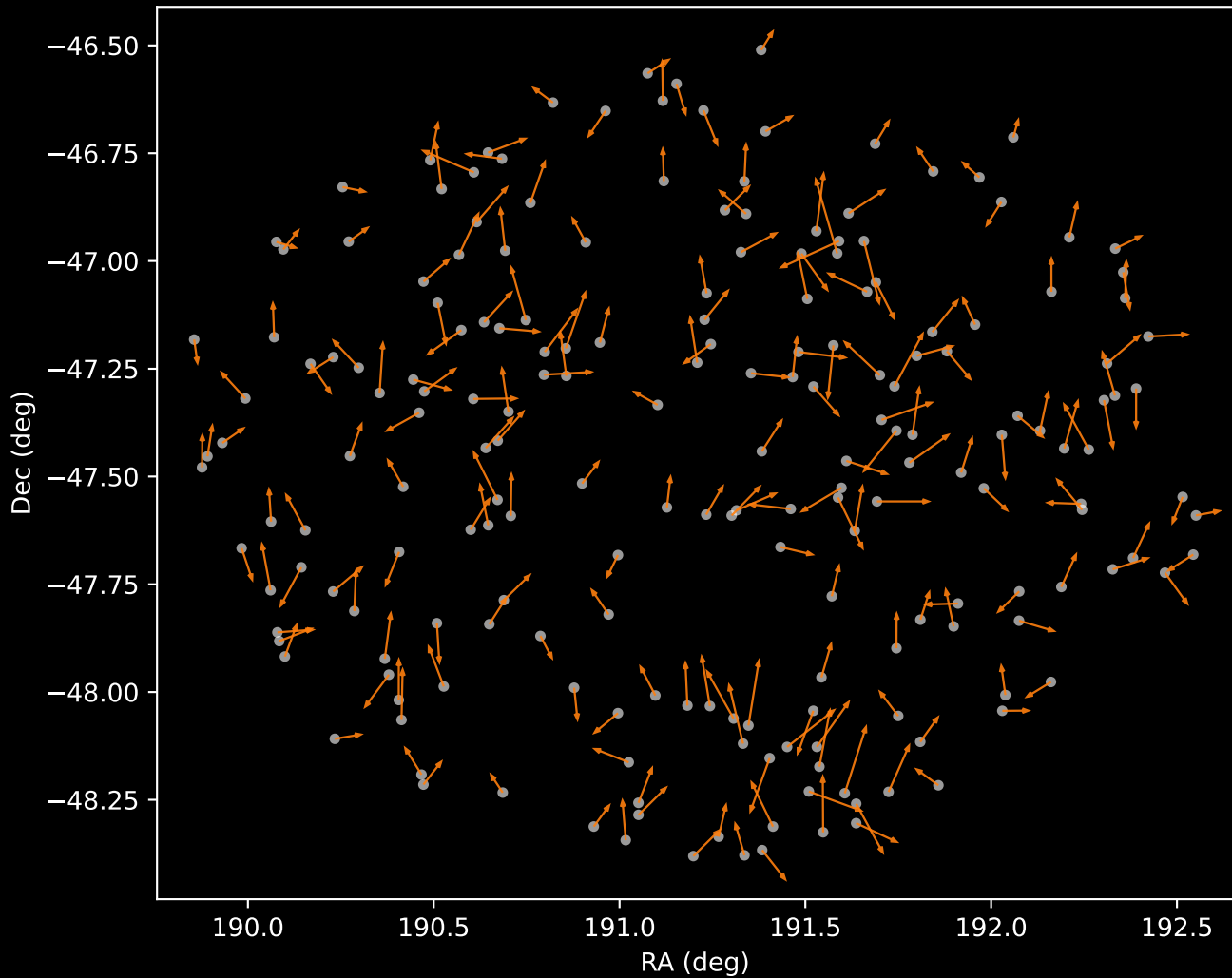
APOGEE DR17 Cluster 2 Proper Motion Vectors (n=203)
