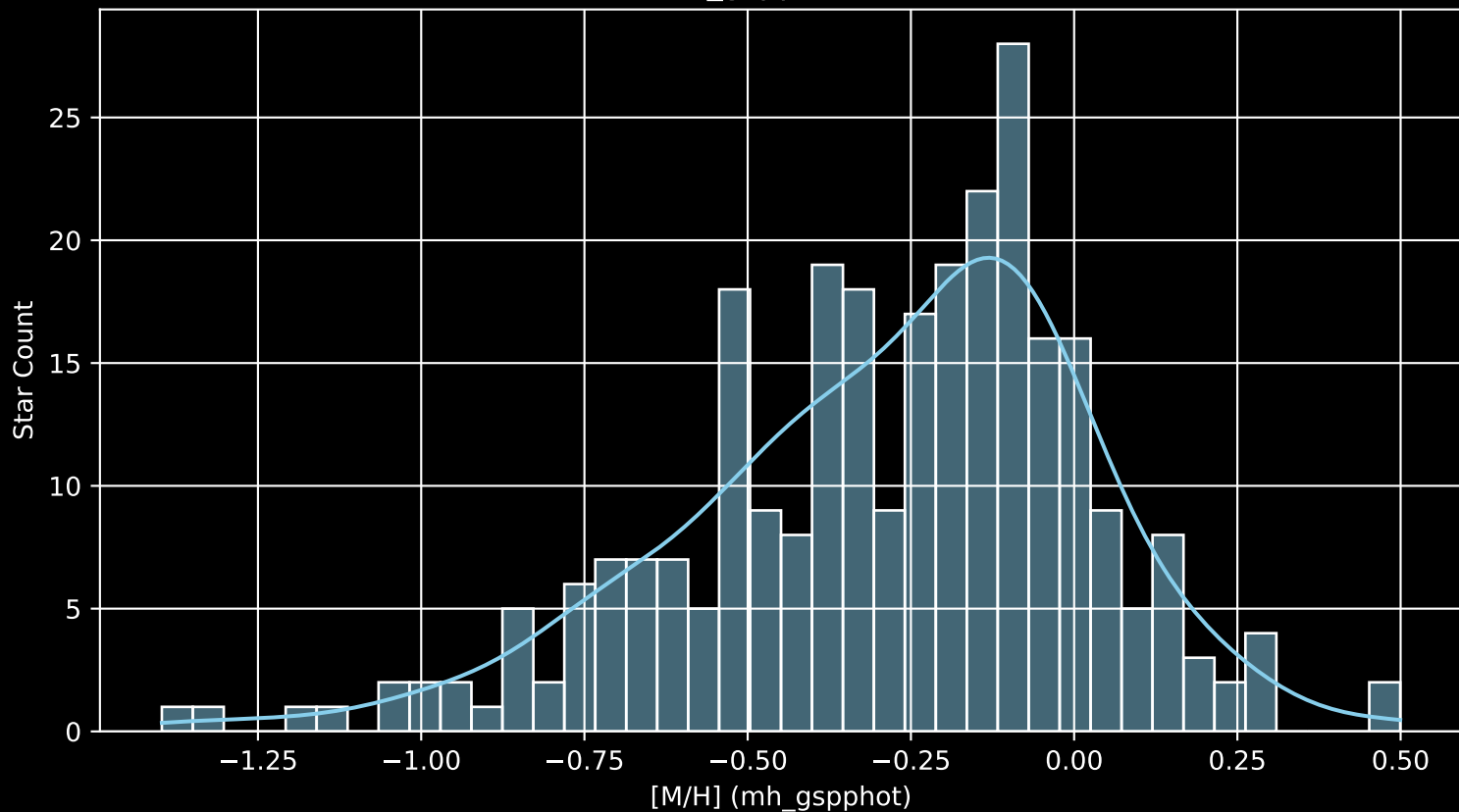
APOGEE DR17 Field: [255-27 [M/H] (mh_gspphot) (n= 282)
