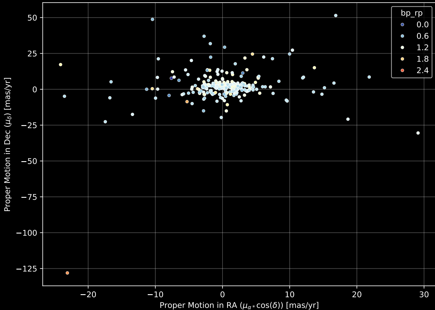
APOGEE DR17 Field: [255-27] Proper Motion Diagram (n= 283)
