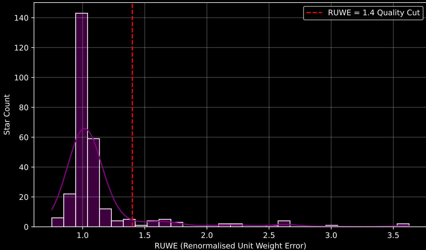
GAPOGEE DR17 Field [255-27] RUWE Distribution (n= 277)
