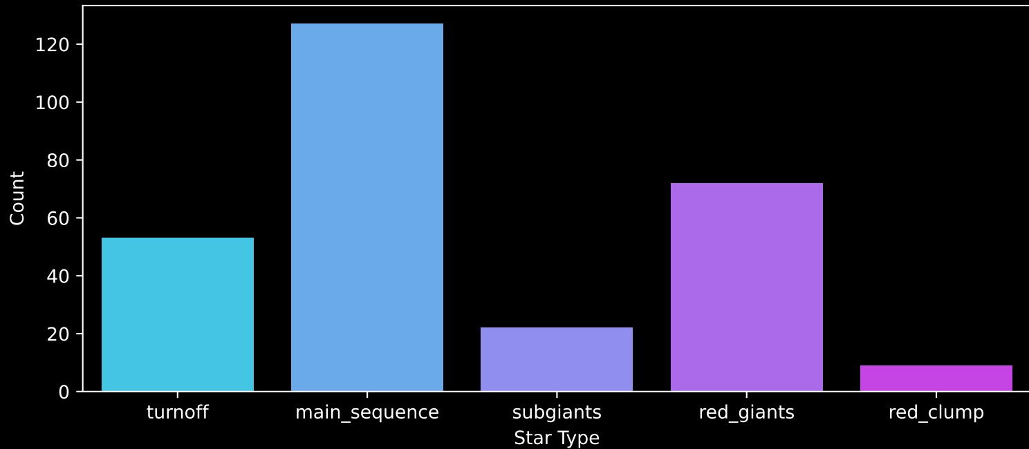
APOGEE DR17 Field: [255-27] Count plot of Star Type
